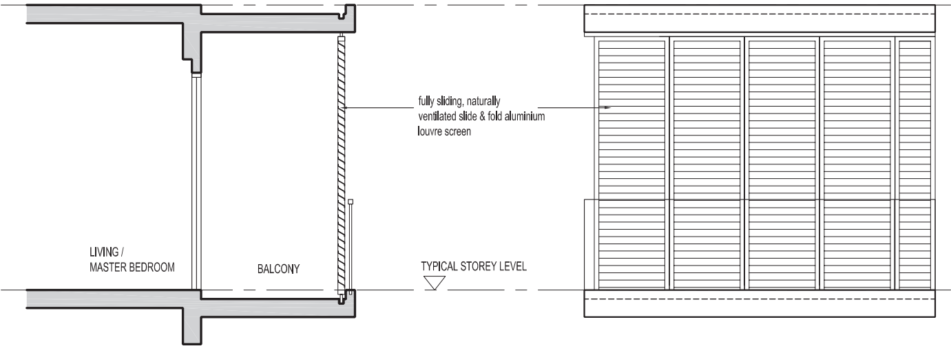
SECTION
