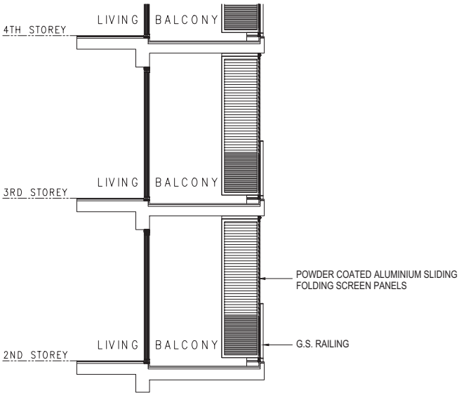
ELEVATION, OPEN POSITION
