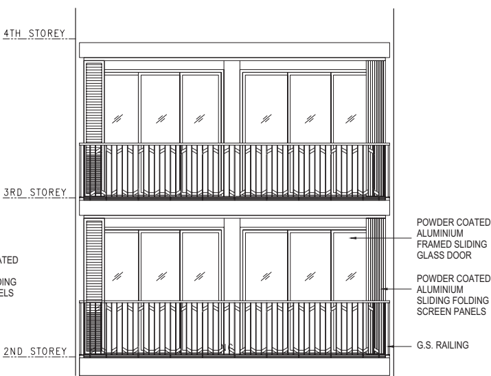
ELEVATION, OPEN POSITION
