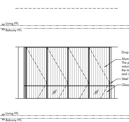
Garden Block Typical Retractable Balcony Screen - Elevation
